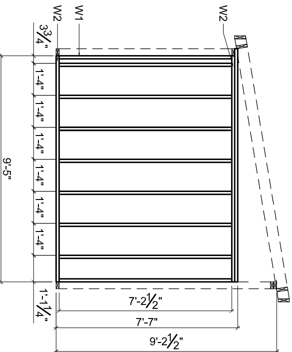
RIGHT WALL FRAMING PLAN
