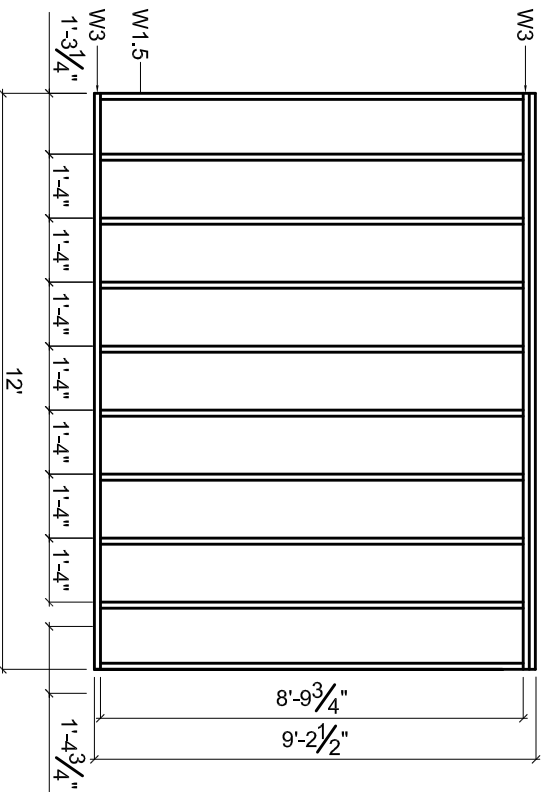
REAR WALL FRAMING PLAN
