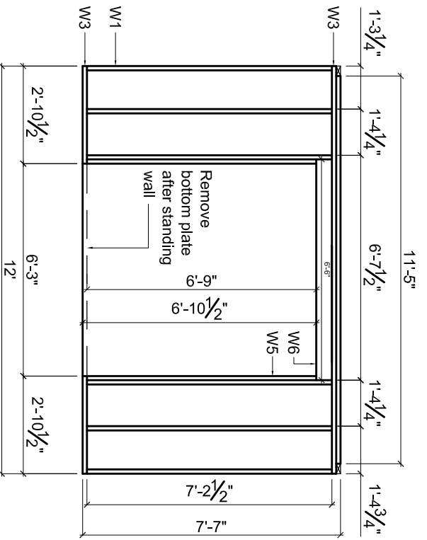
FRONT WALL FRAMING PLAN
