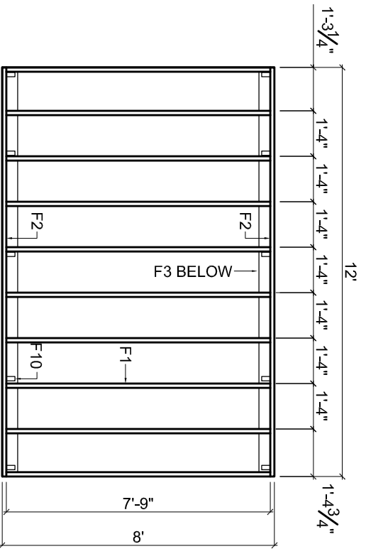
FLOOR FRAMING PLAN
