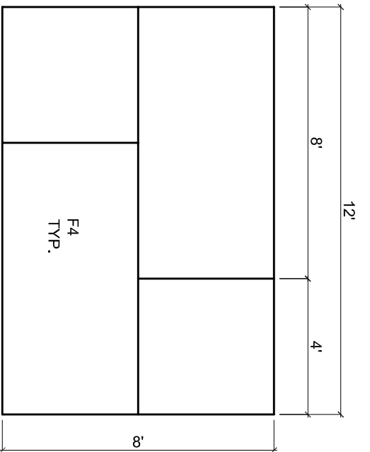
FLOOR SHEETING PLAN
